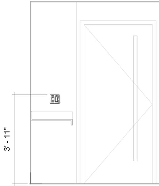
① 1/2" = 1'-0"
