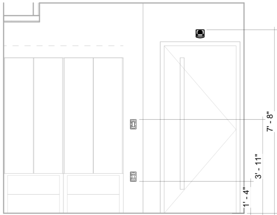
⑤ 1/2" = 1'-0"
