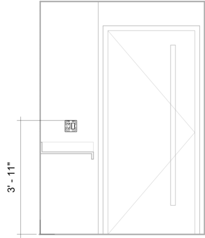
① 1/2" = 1'-0"
