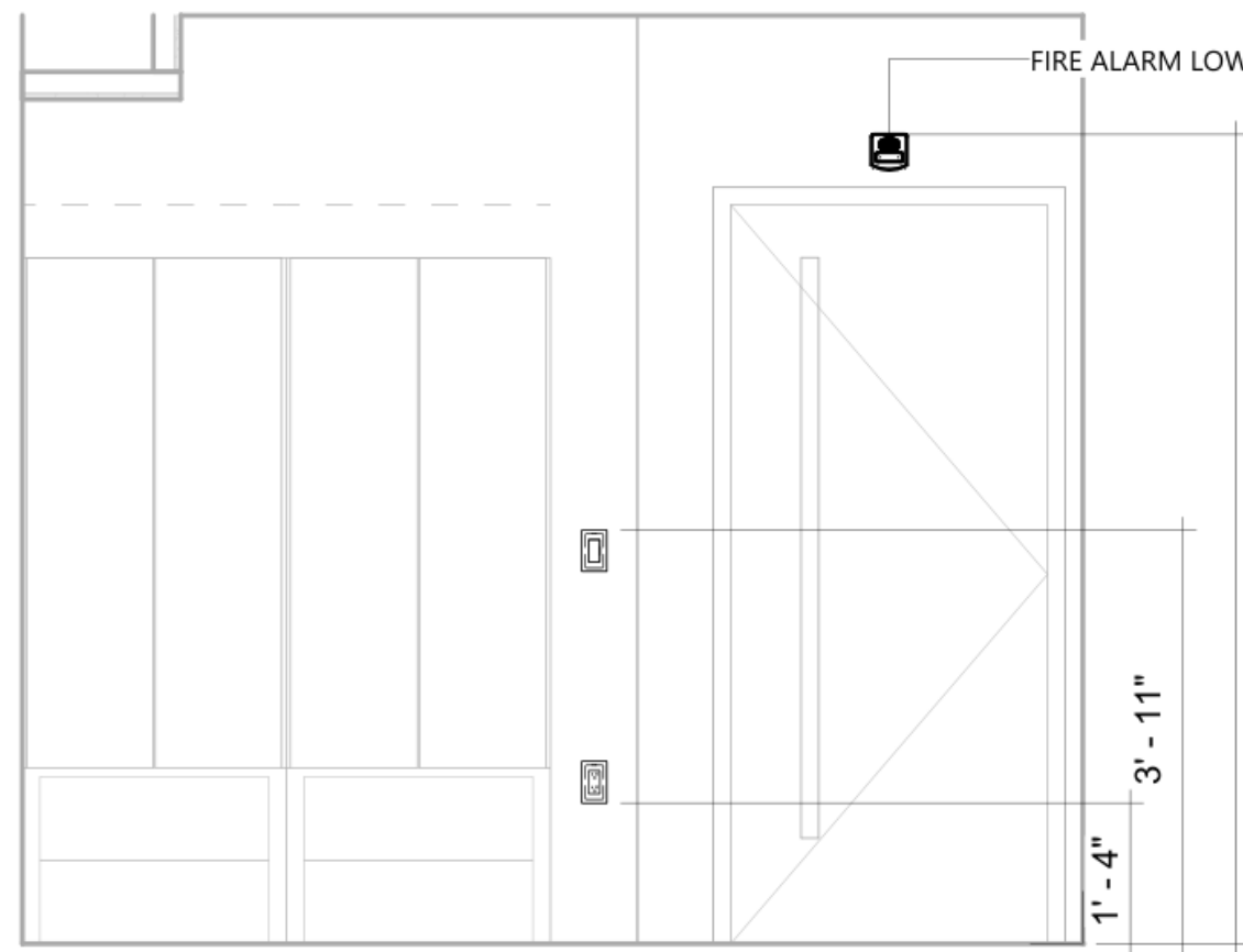
⑤ 1/2" = 1'-0"
